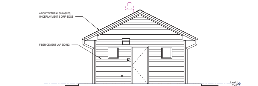
2 BUILDING ELEVATION 1/8" = 1'-0"
