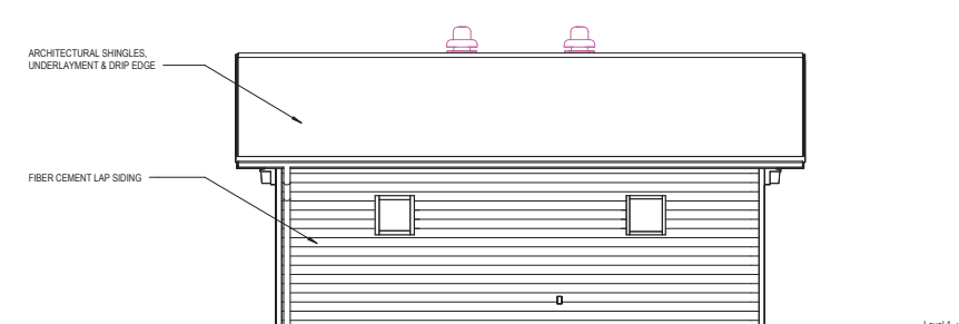
4 BUILDING ELEVATION 1/8" = 1'-0"
