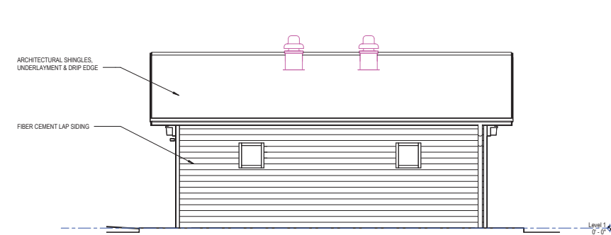
1 BUILDING ELEVATION 1/8" = 1'-0"
