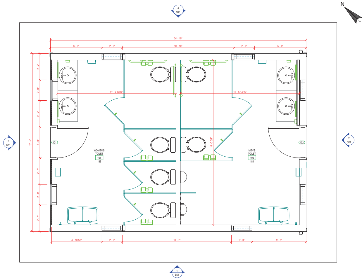
FLOOR PLAN NOTED 1/2" = 1'-0"
