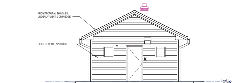
3 BUILDING ELEVATION 1/8" = 1'-0"
